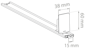
26 FORTA NORMA-0 Pusher without front
