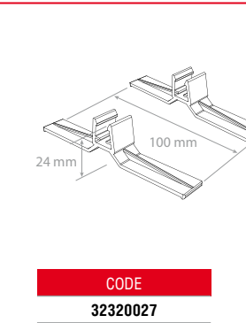
BASE-90 Support clip
