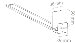
28 FORTA NORMA-2 Pusher with a front riser
