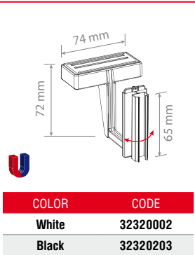
MAG-FLEX-PF Vertical plastic frame holder with strong magnet
