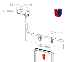
MAG-SW-TUBE-L-PF Magnetic sign holder with angle adjustment
