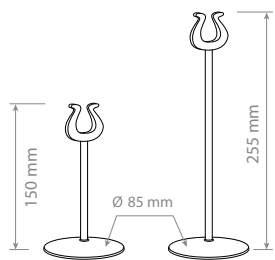
MV-CLIP-XL Fenix shape metal price holder
