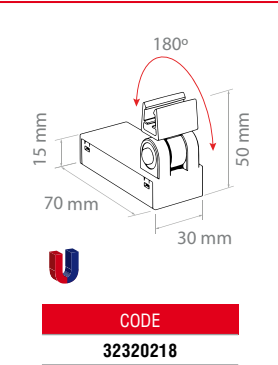
MAG-SW-PF Adjustable magnetic frame holder
