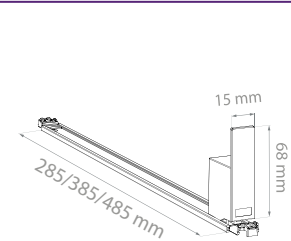
FORTA SLIMA-0 Slim pusher with high back support
