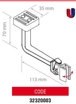
MGT-SW Swivel magnetic holder
