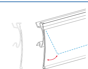
HSAC Flip-up price label holder for shelves with 25mm C-channel
