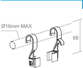
EZ-PF-HOOK Plastic frame suspension hook for EZTRACK
