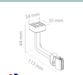
MGT-SW-SUPERGRIP Swivel magnetic sign holder
