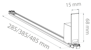
29 FORTA SLIMA-0 Slim high pusher with no front
