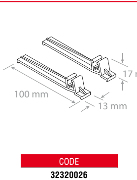
BASE-75 Support clip
