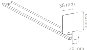
27 FORTA NORMA-1 Pusher with a small front
